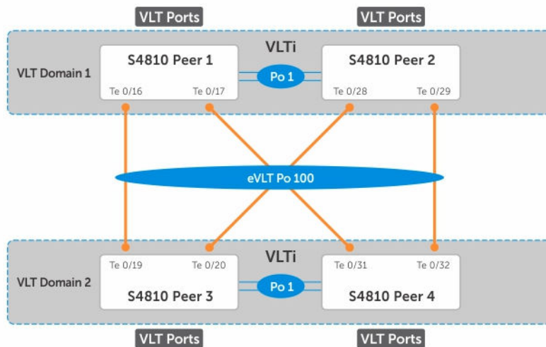
Figure 121. eVLT Configuration Example
